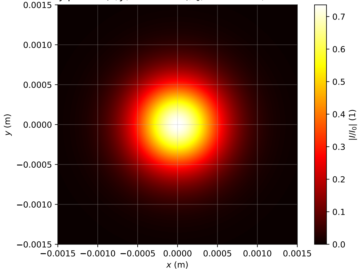
Intensity profile I(x, y, z = 2.309m)/I_0 , Pin=0.5Pcr, artificial time
